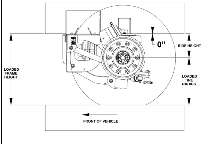
FRAME KIT 8A000491
