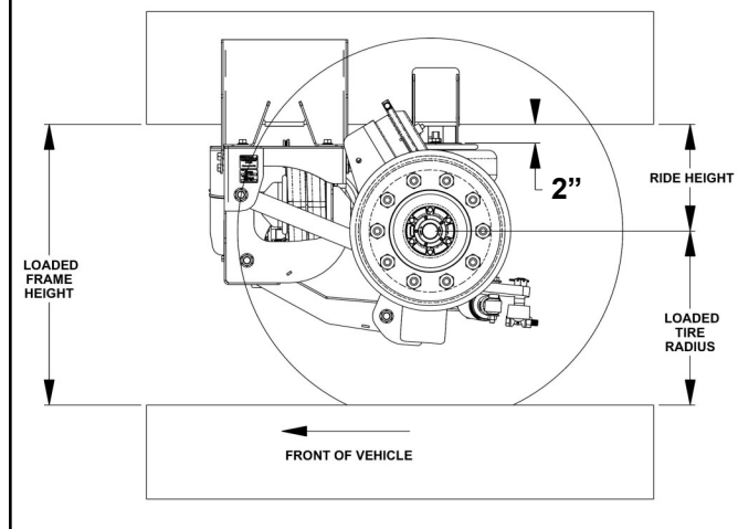
FRAME KIT 8A000492
