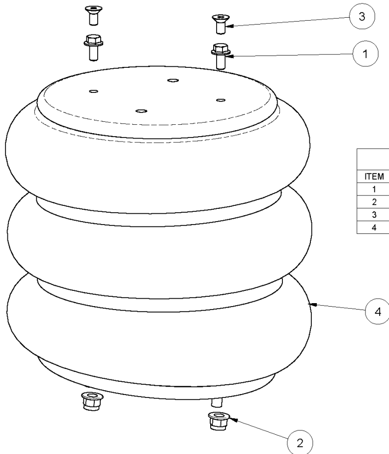
4AS00070 - SERVICE KIT - LOAD SPRING
