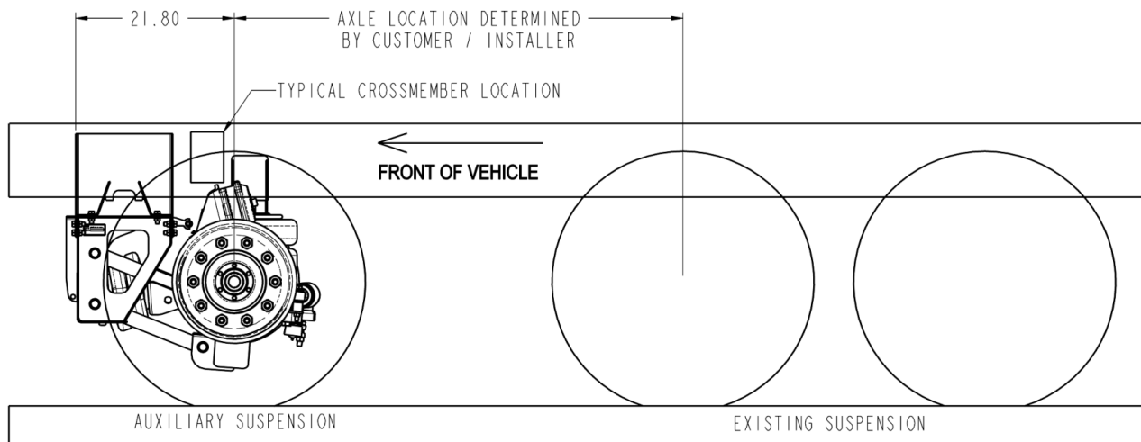
PUSHER CONFIGURATION
