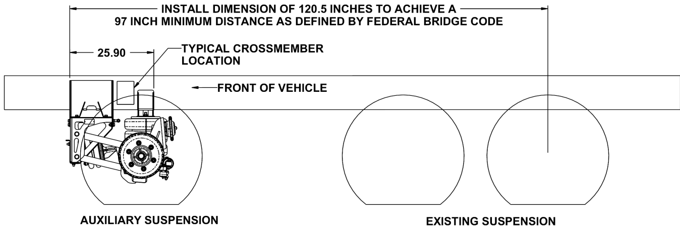
PUSHER CONFIGURATION
